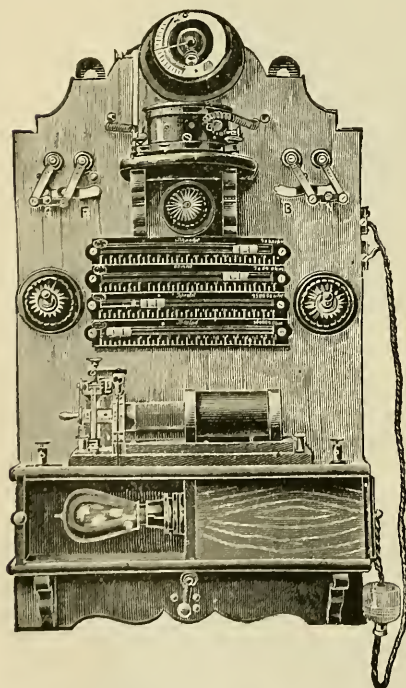
FIG. 114. — Switch board for regulating lighting currents by means of resistances.
